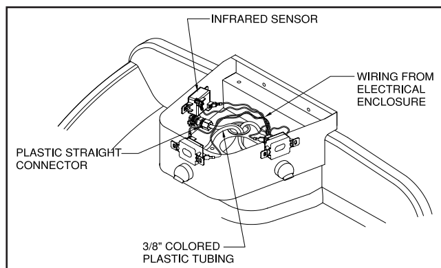
Infrared Sensor
